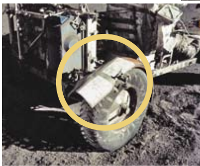
Lunar rover wheels stirred up so much dust (above) that makeshift dust fenders had to be added (left).
