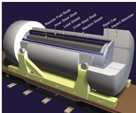
Figure 6 (below) Once cooled, the rod stacks would be housed in 125-ton steel canisters for transport to Yucca Mountain for storage.
