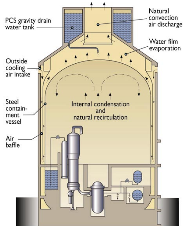
Figure 3 New “passive safety” reactor designs use such natural forces as gravity, circulation, condensation, and evaporation to react automatically to accidents without operator intervention.
