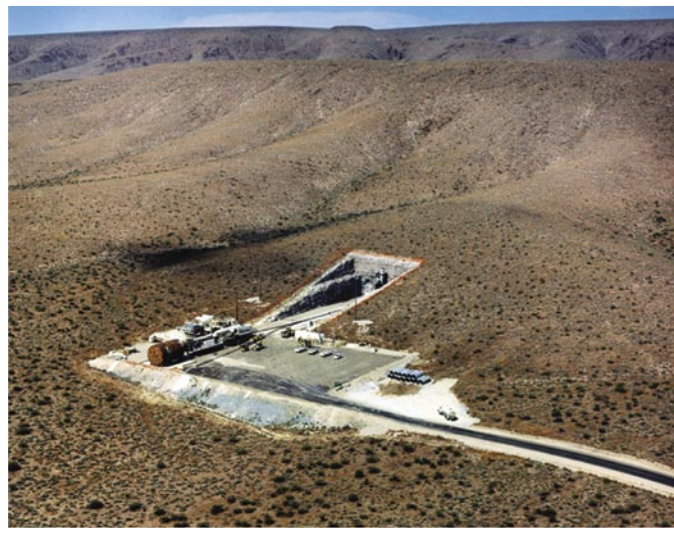
Figure 7 View of the south portal of the Yucca Mountain exploratory studies facility, showing the 25-foot-diameter tunnel boring machine.
